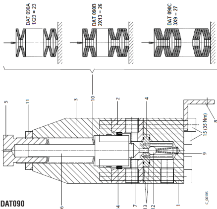
DAT 090 PRESSURE REDUCING PART NUMBERS
